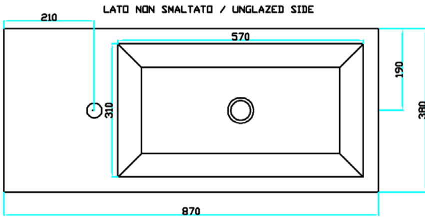
VISTA FRONTALE / FRONT VIEW
