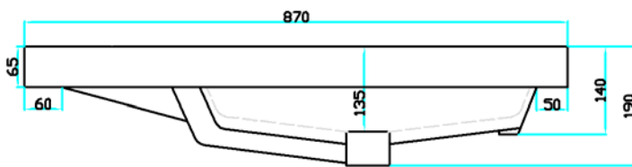
VISTA FRONTALE / FRONT VIEW
