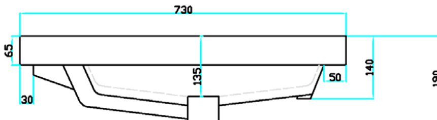
VISTA FRONTALE / FRONT VIEW
