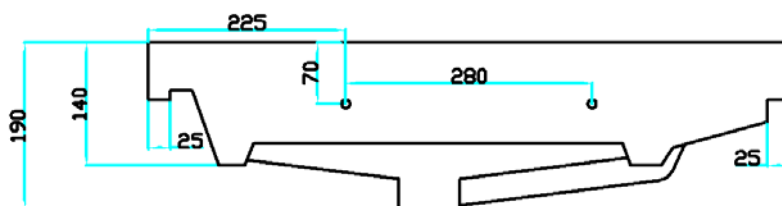
VISTA POSTERIORE / BACK VIEW
